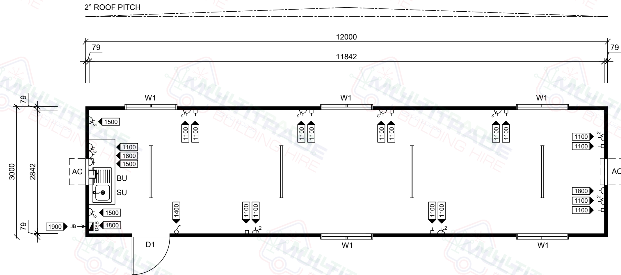
12.0x3.0m Crib Room - Floor Plan
